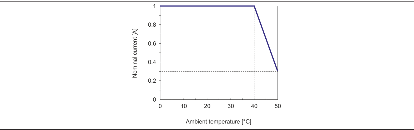
Figure 6: Current derating
