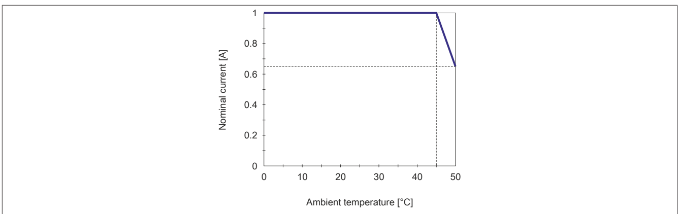
Figure 4: Current derating
