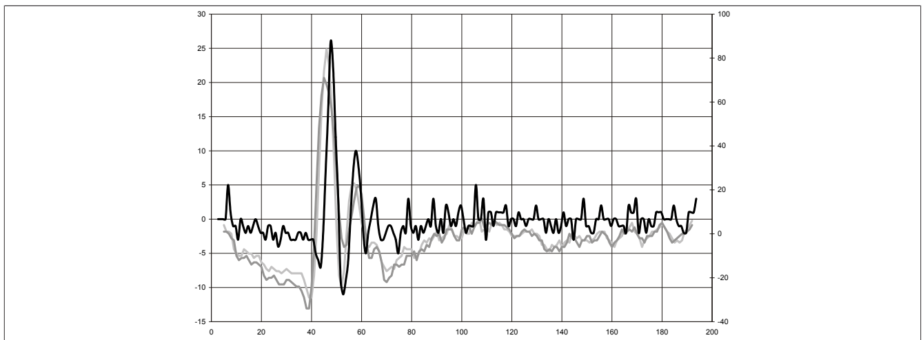
Figure 4: Example 1 - Calculated curvature (2nd derivative) of the current curve including overlapping sum with 3 different window widths
