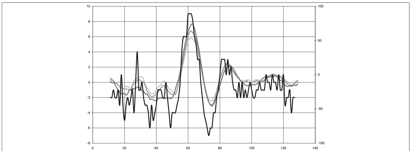
Figure 7: Example 2 - Calculated curvature (2nd derivative) of the current curve including overlapping sum with 3 different window widths
