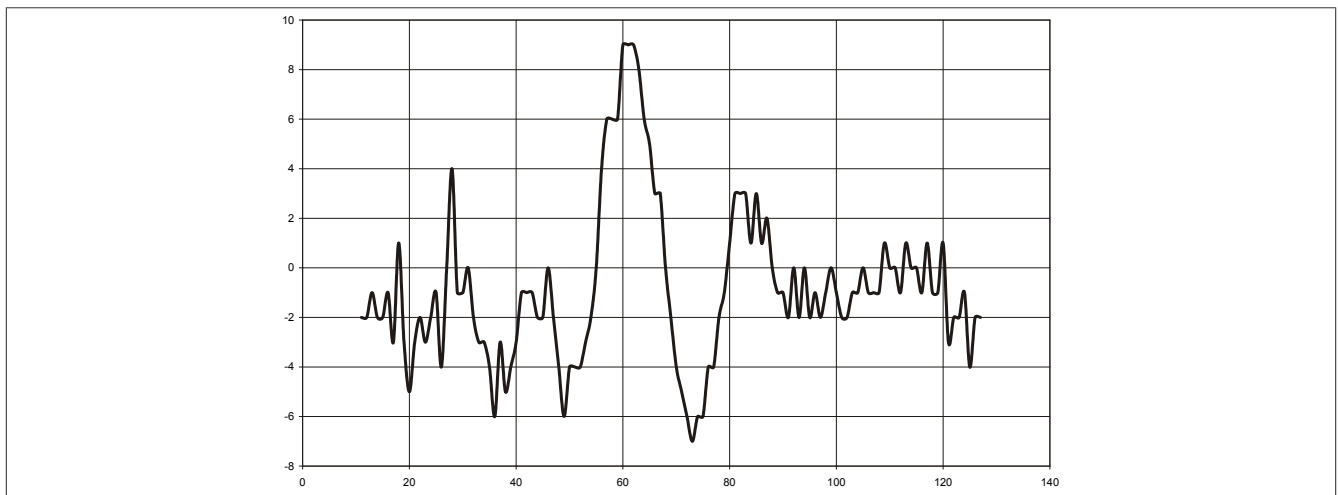
Figure 6: Example 2 - Calculated curvature (2nd derivative) of the current curve
