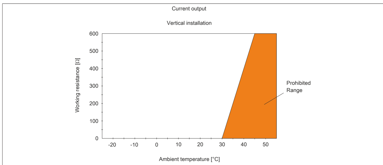
Figure 4: Derating the load with a current output and vertical mounting
