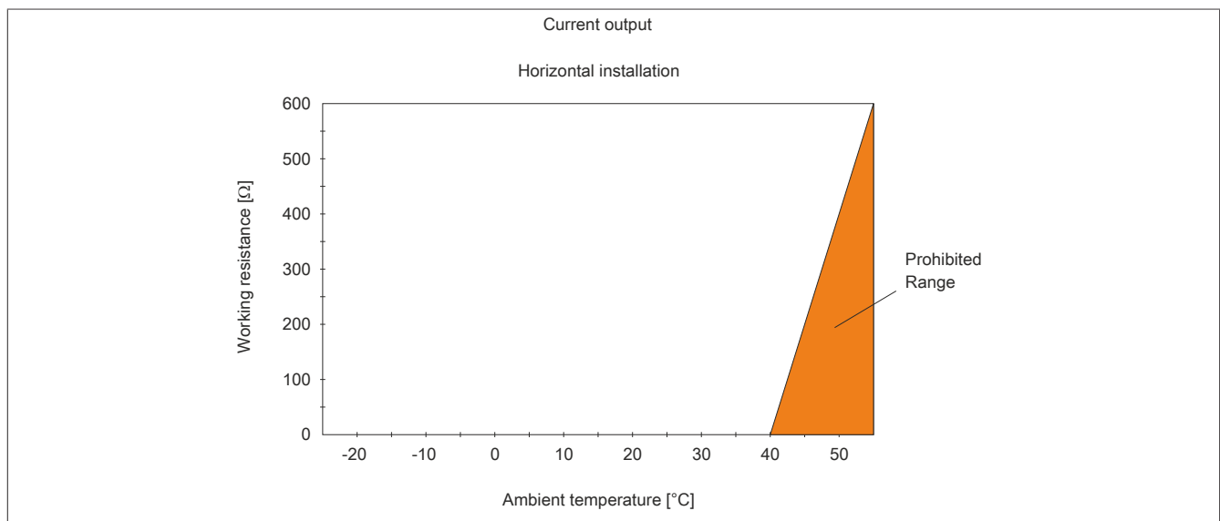
Figure 2: Derating the load with a current output and horizontal mounting
