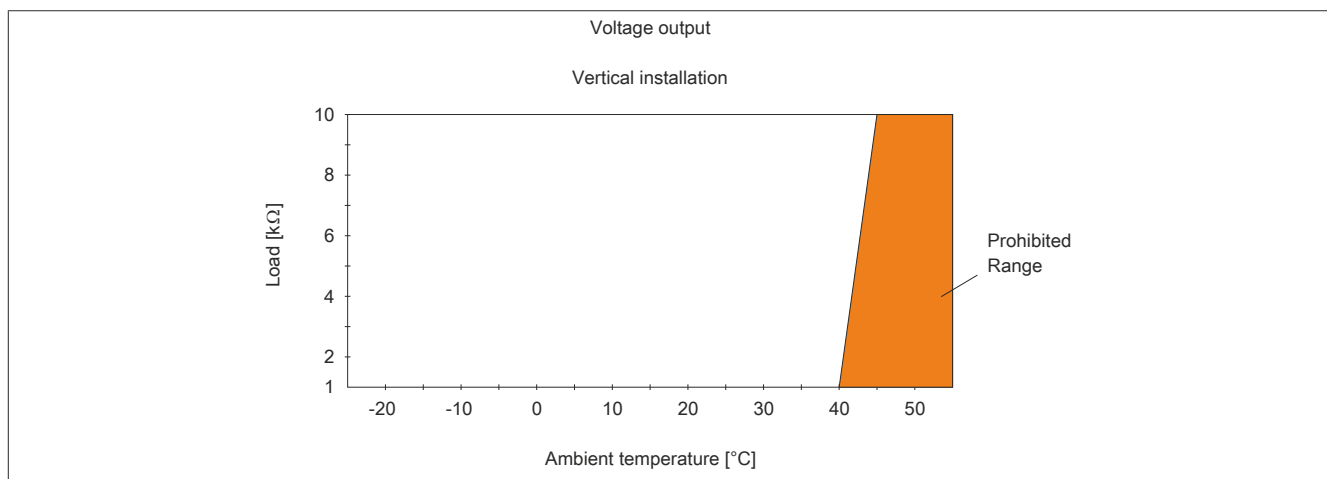
Figure 3: Derating the load with a voltage output and vertical mounting
