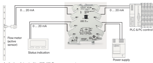
Application of signal splitter 857-423: Flow measurement
