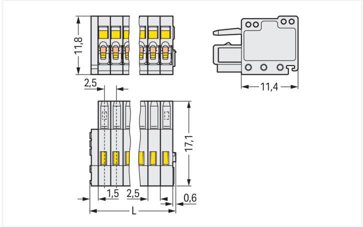
Dimensions in mm L = (pole no. x pin spacing) + 2.1 mm
