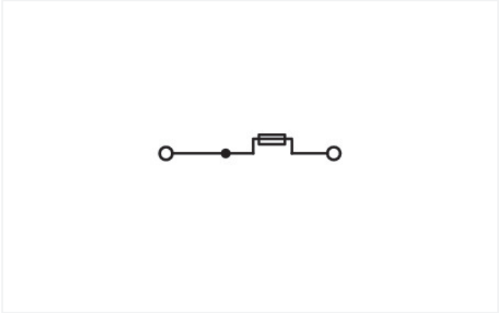
Fuse terminal block, 282 Series, CAGE CLAMP®
