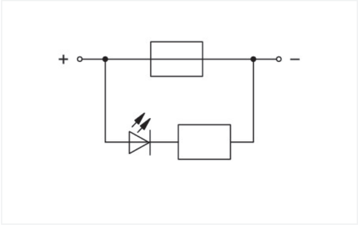
Fuse terminal block, 282 Series, operating tool
