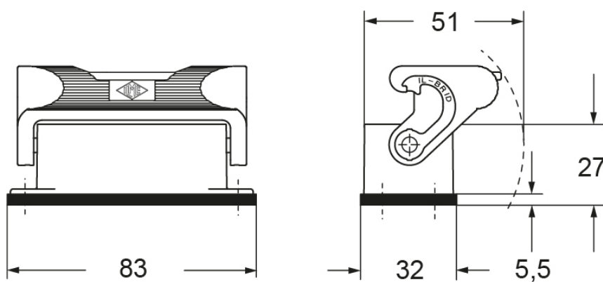
Catalogue drawings
