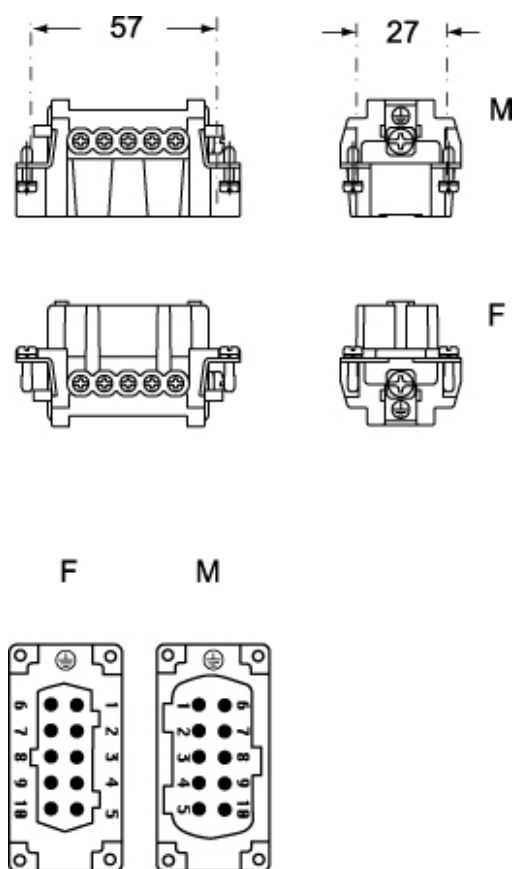
Catalogue drawings
