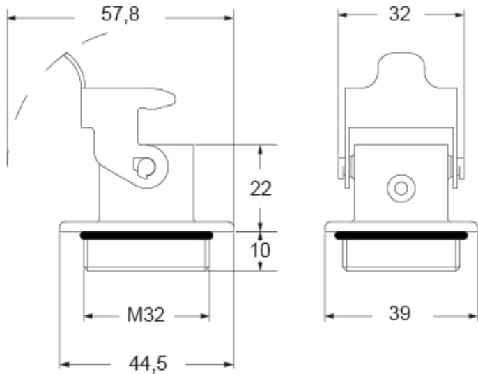
Catalogue drawings
