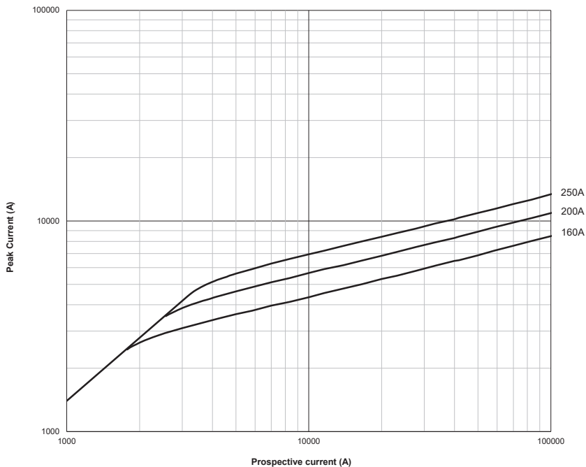
Cut-off curve - Size 2, 160 A to 250 A
