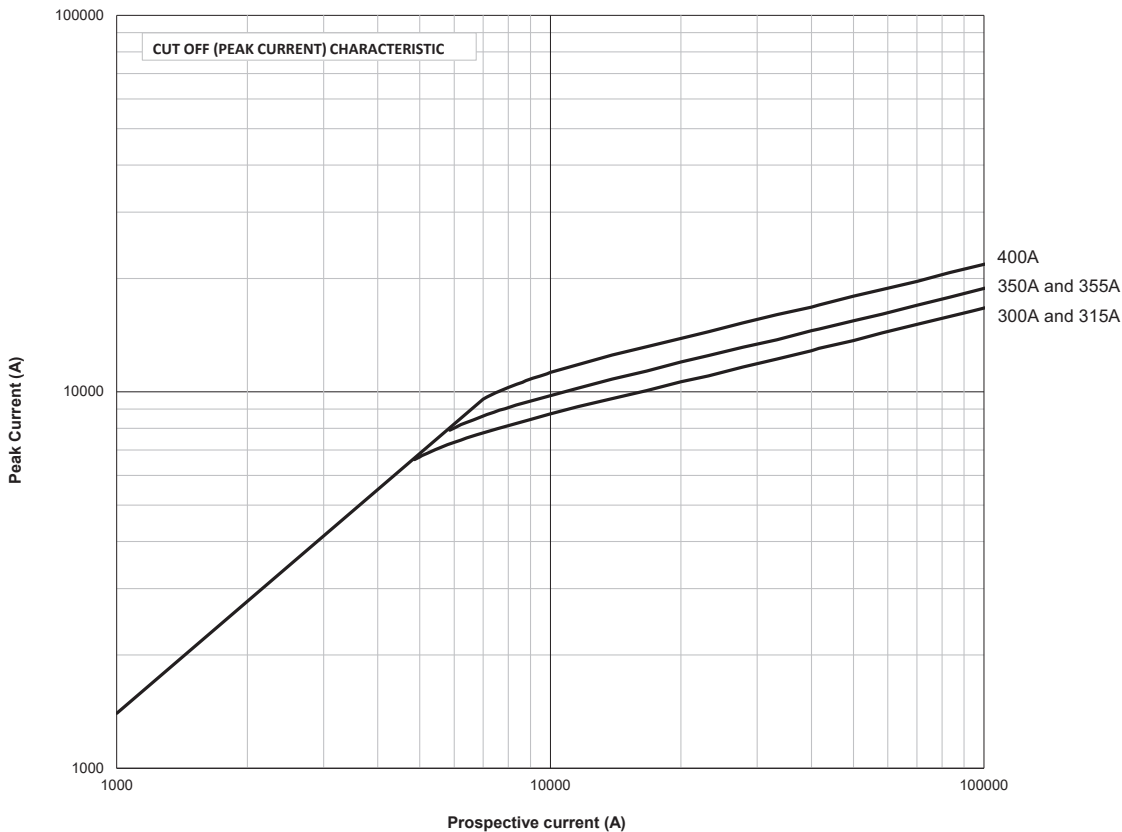
Cut-off curve - Size 3, 300 A to 400 A
