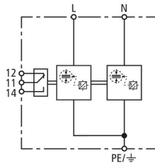
Basic circuit diagram DSH TN 255 FM
