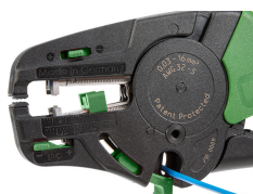
Cutting a conductor.
