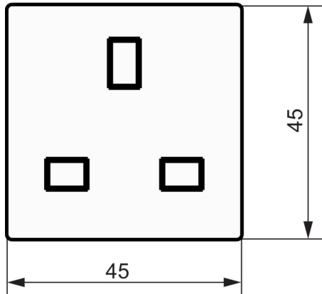
Dimensioned drawing
