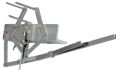
bench mounted sleeving tool D1/2-01
